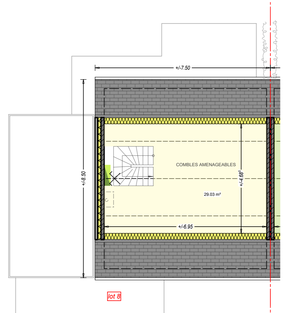
PLAN COMBLES
