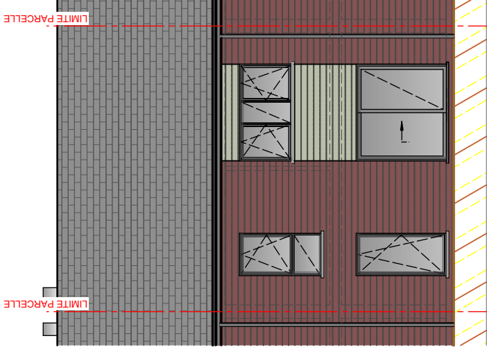
lot 4 FACADE ARRIERE
