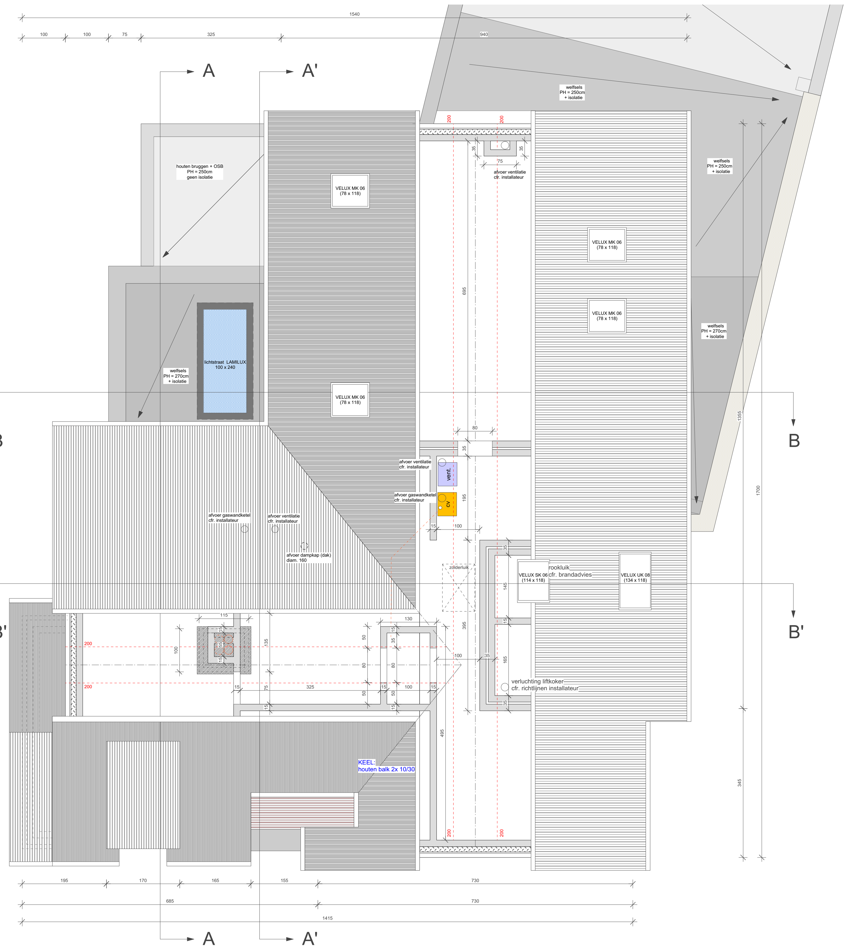
ZOLDER 1/50
