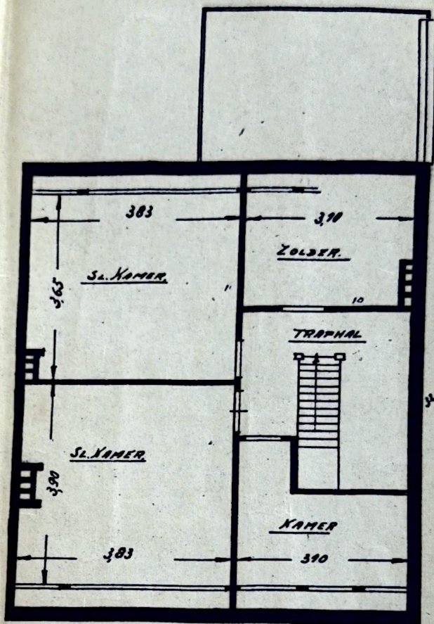
ZOLDER PLAN.
