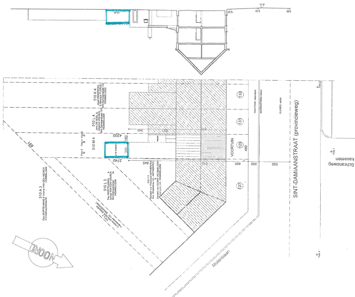
INPLANTING (1/200)
