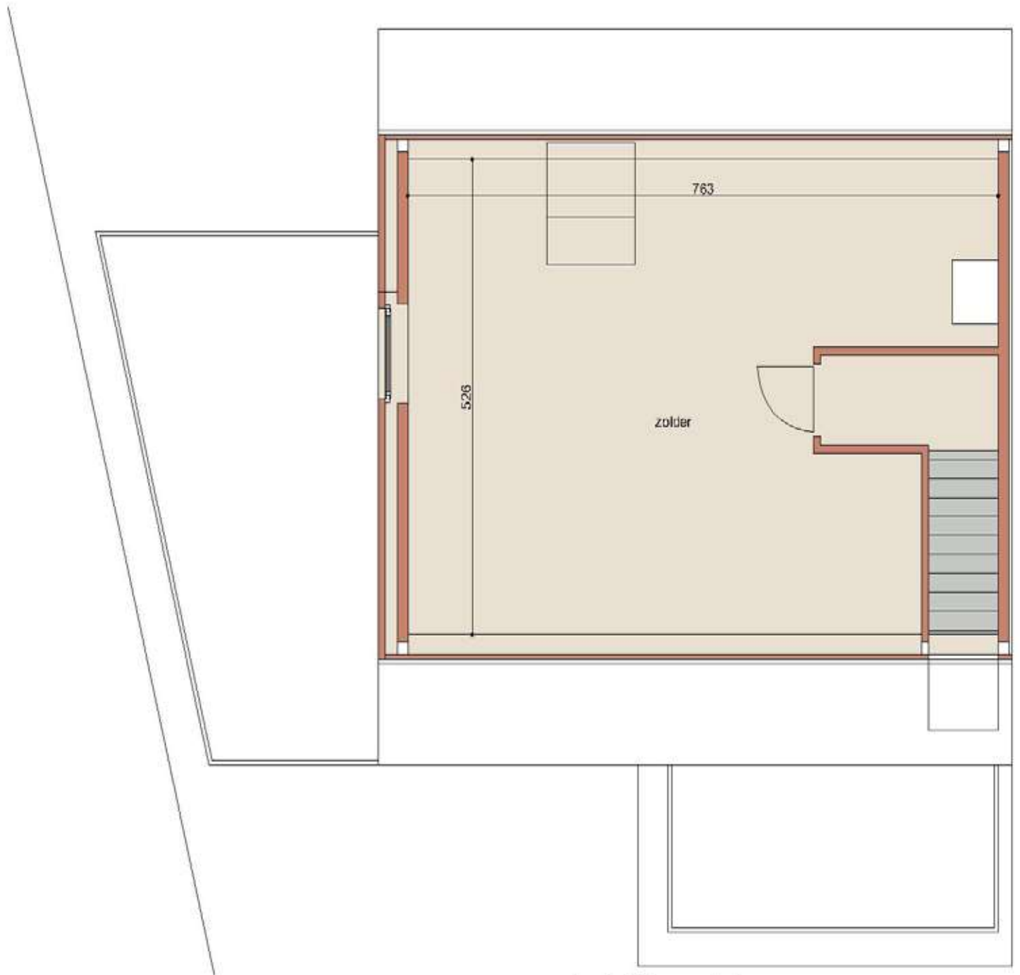
lot 3 zolder
