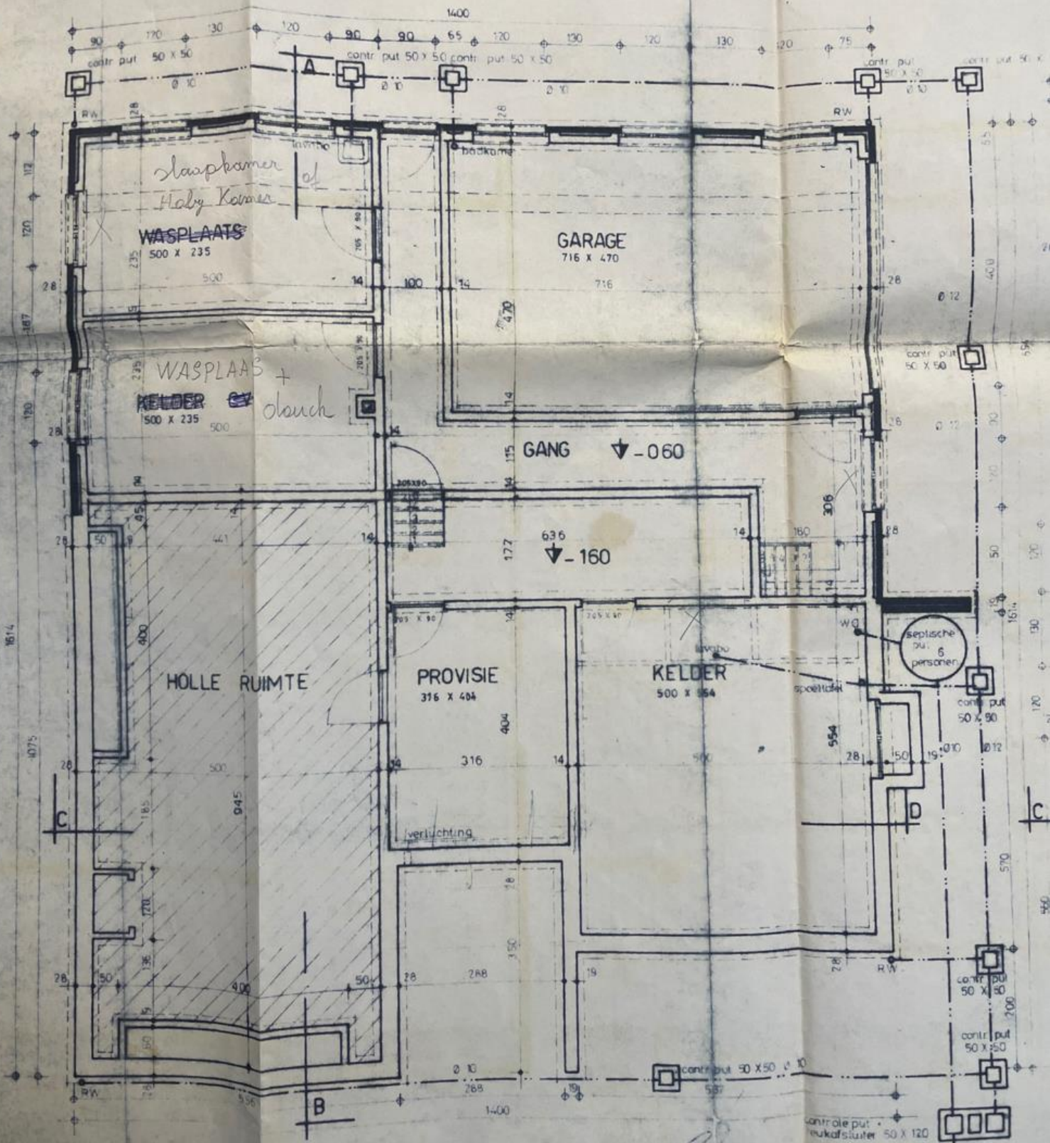
PLAN KELDER - RIOLERING
