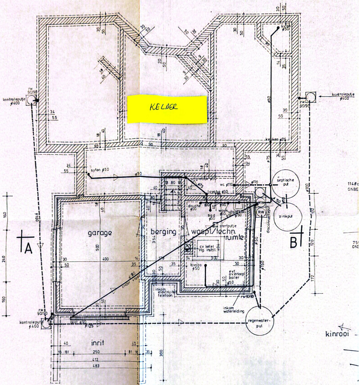
kelder/funderings-en rioleringsplan 1/50
