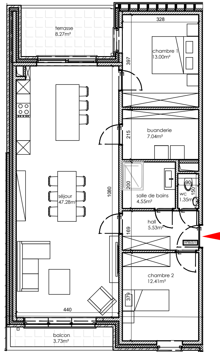
Plan Ech: 1/100
