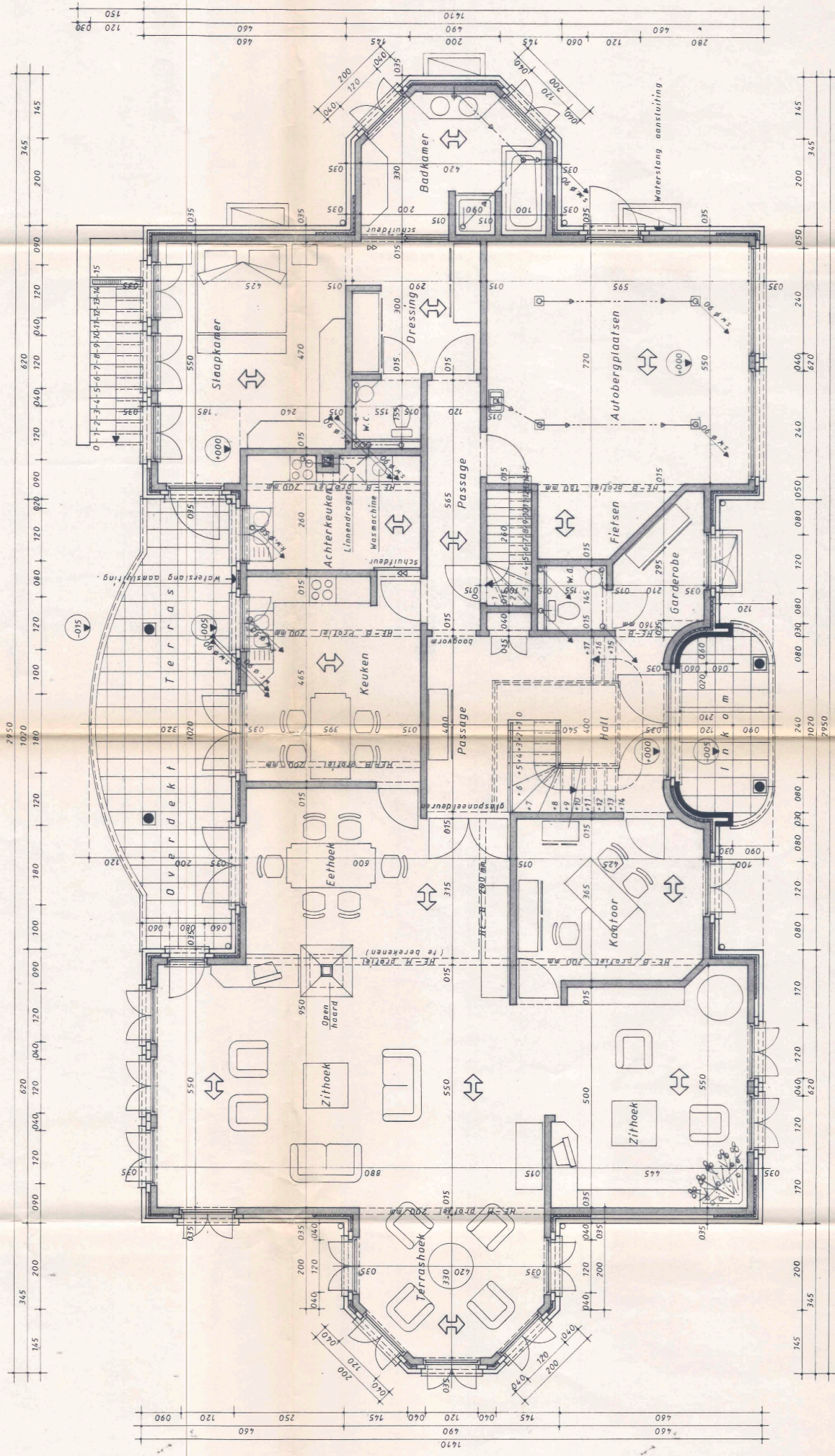
Plan begane grond □ Nivo 0.00 m □
