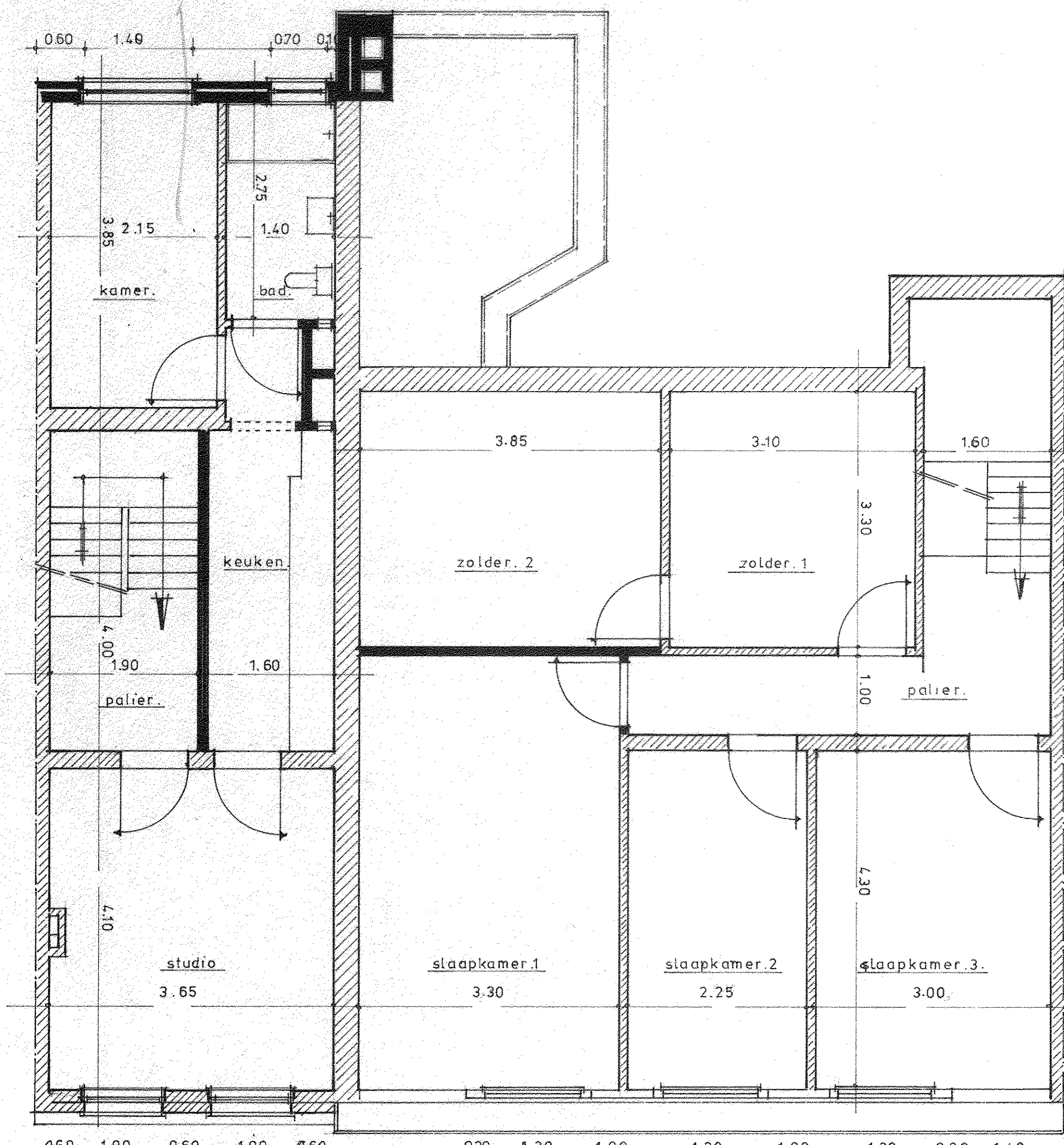
plan: zolder.
