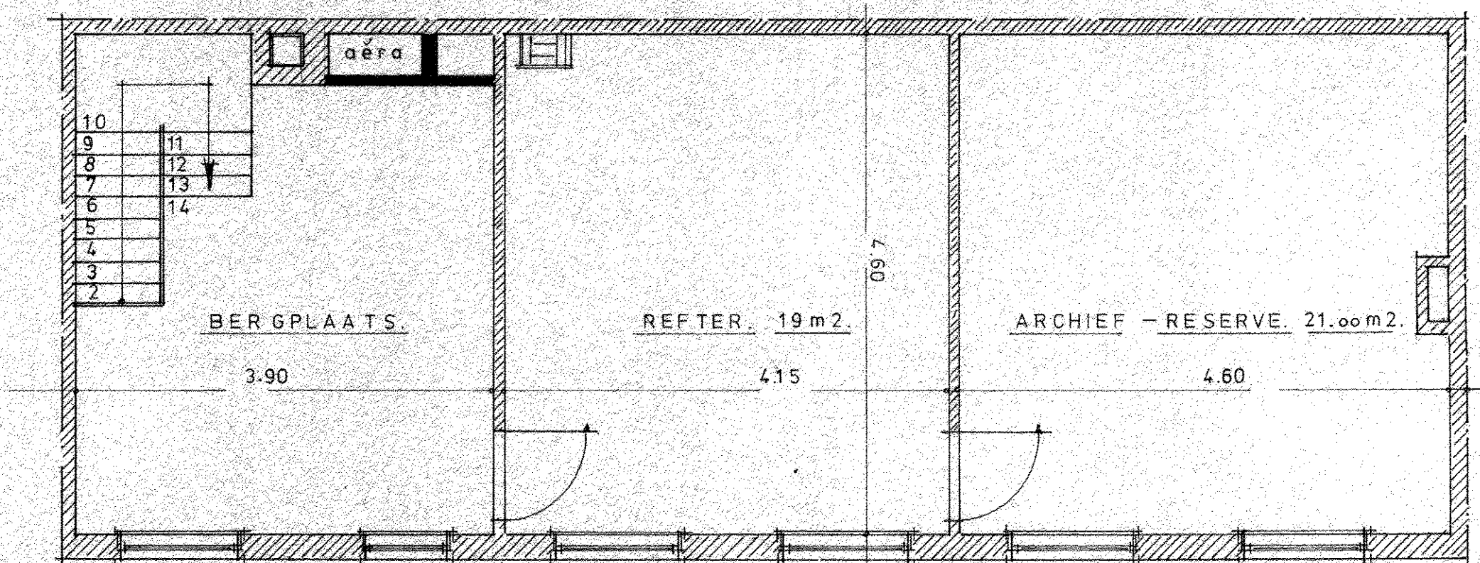
1. verdieping.
