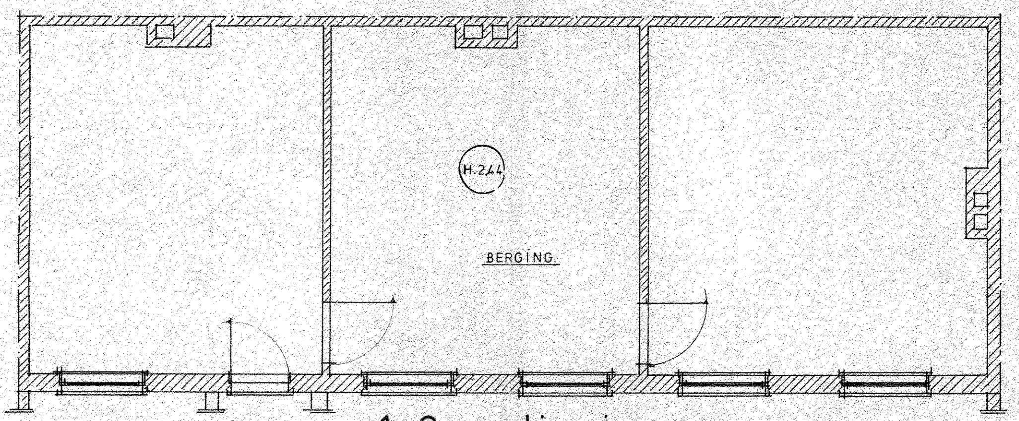
1-2 verdieping.
