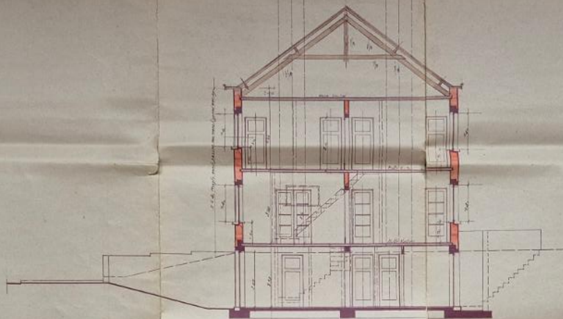
DOORSNED.
