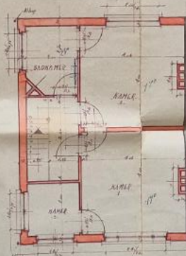
VERDIEPING.
