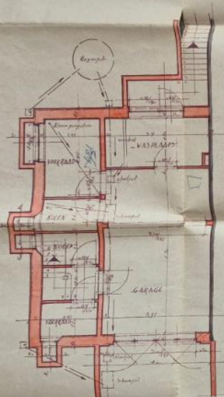
-KELDERING-
