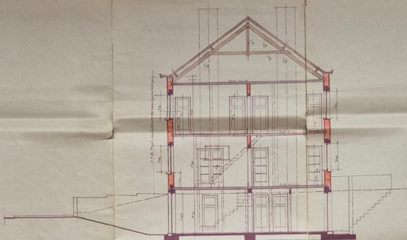
-DOORSNED-
