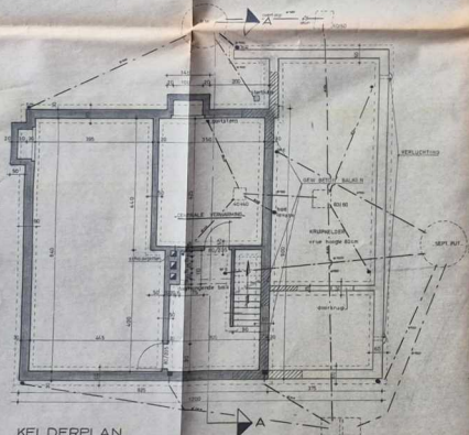
KELDERPLAN
