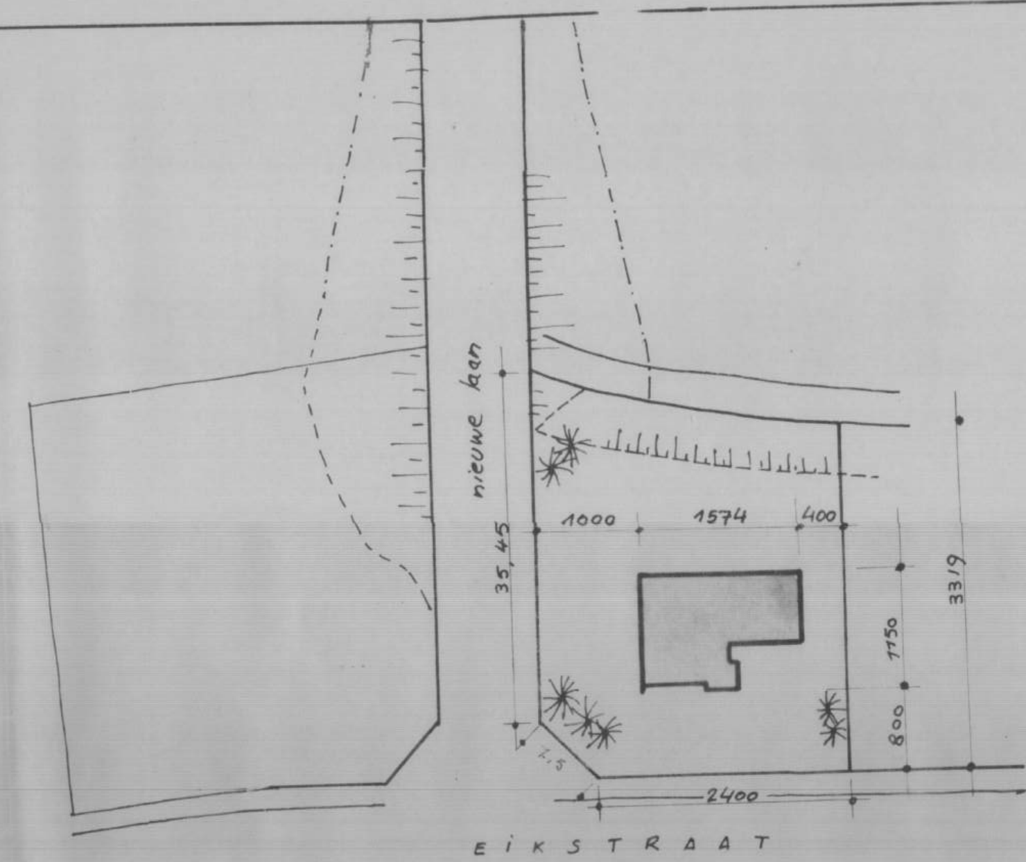
implantingsplan 1/500
