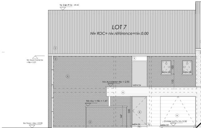
Façade avant_ 1/75
