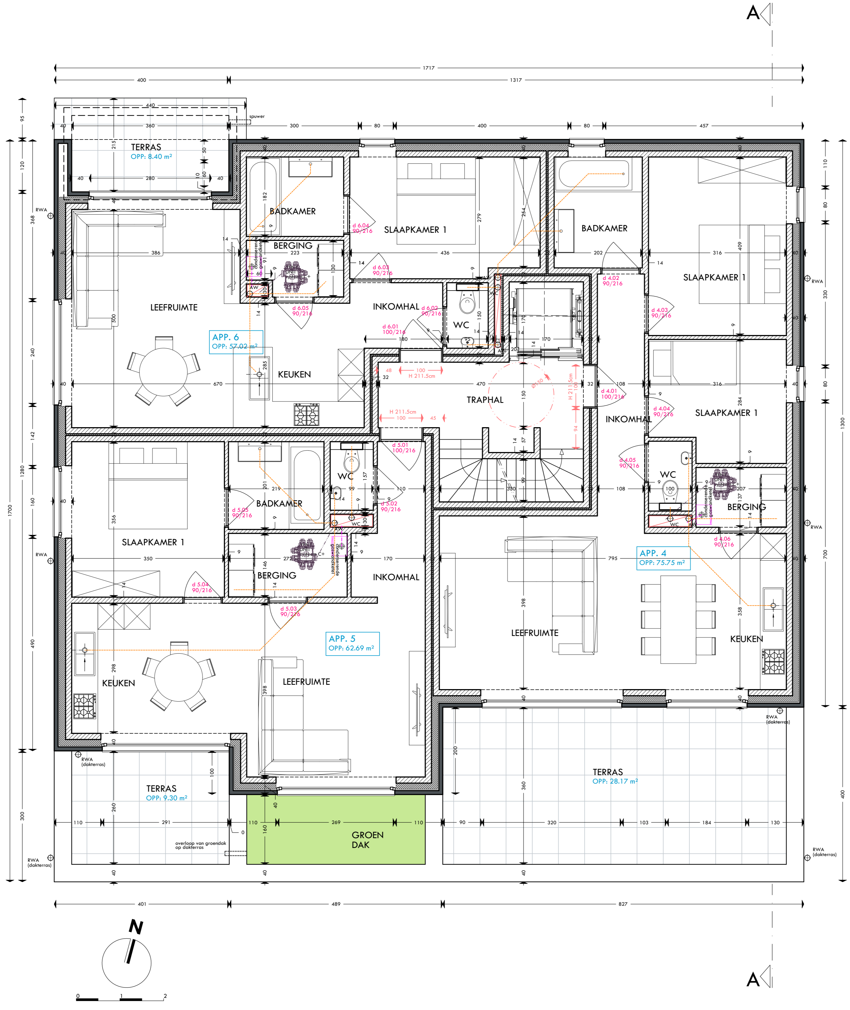
GRONDPLAN VERDIEPING +1
