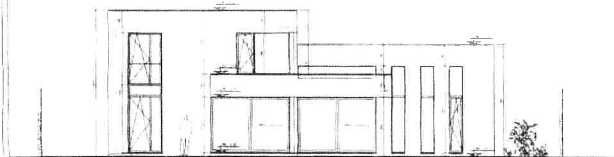
ELEVATION ARRIERE - 1/50ème
