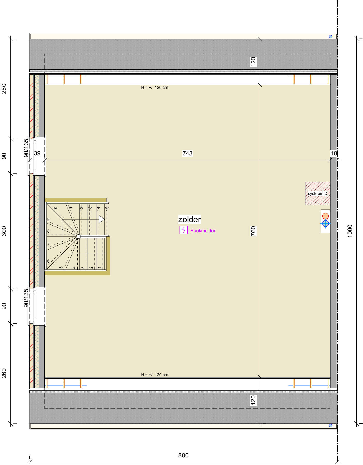
Plan ZOLDERVERDIEPING
