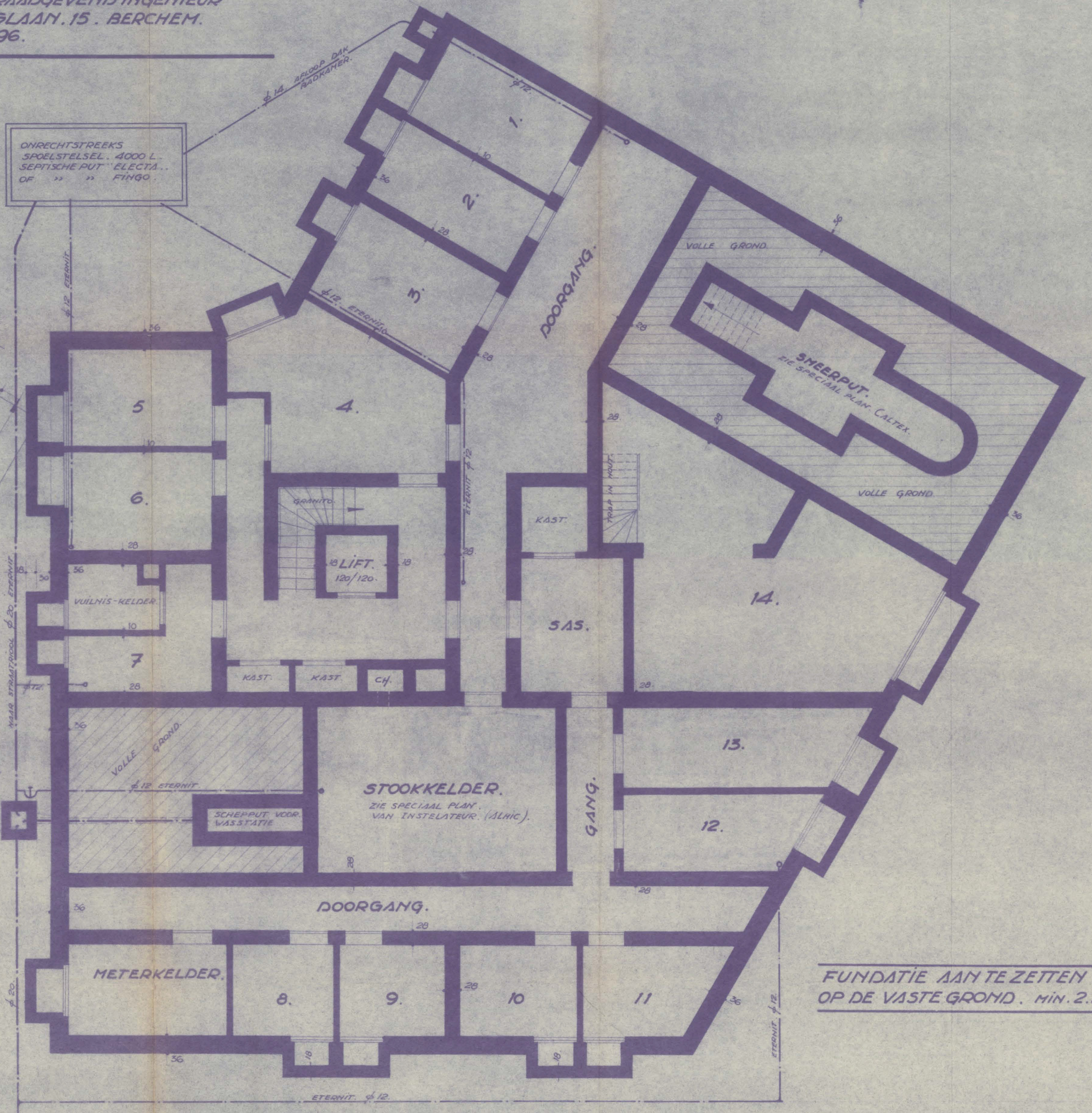
FUNDERING.
