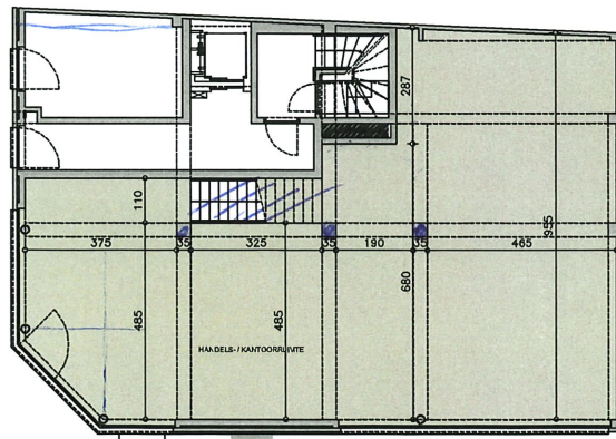
plan nivo 0
