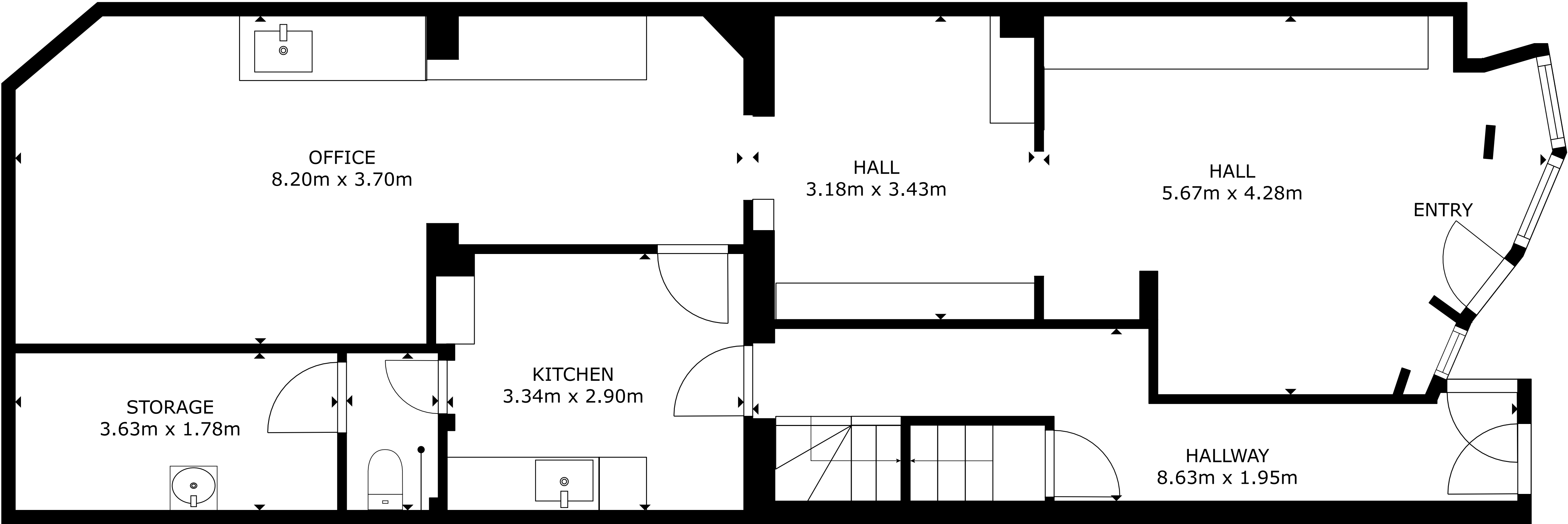
FLOOR 2
