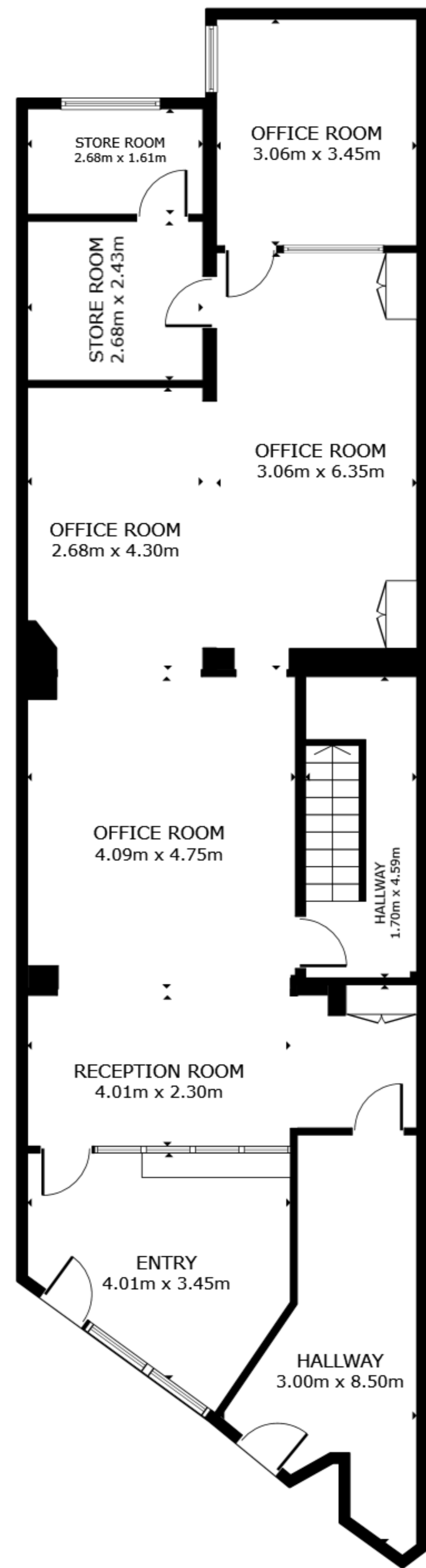
GROUND FLOOR
