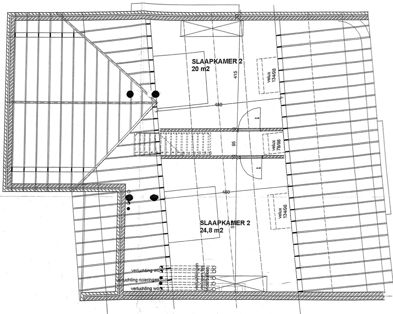
ZOLDERPLAN
