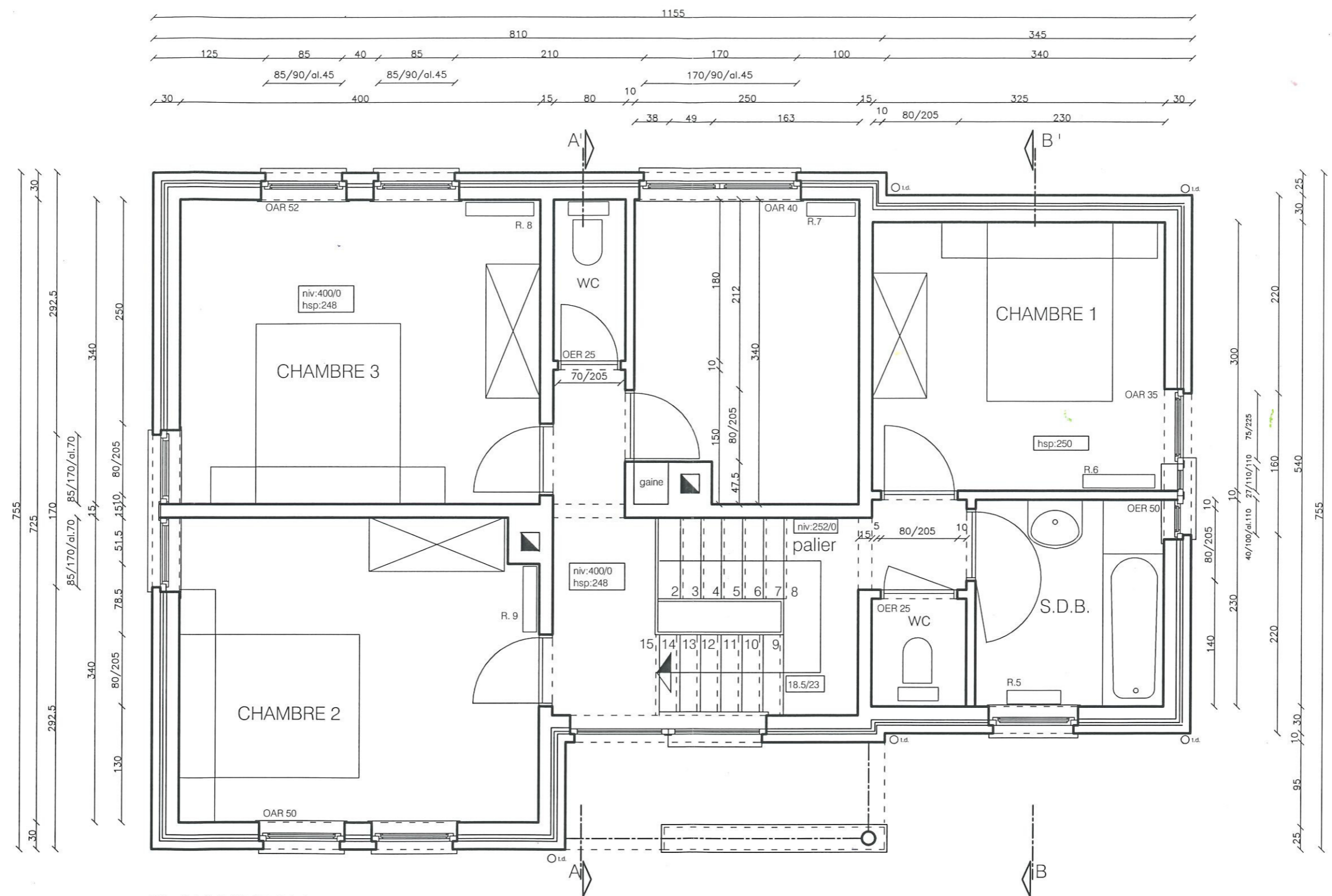
PLAN NIVEAU +1
